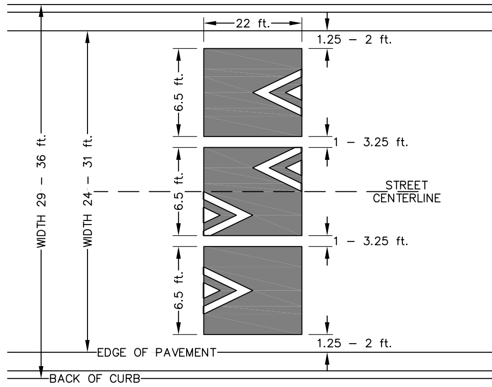
SPEED CUSHION DETAIL
