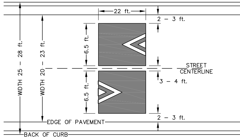
SPEED CUSHION DETAIL
