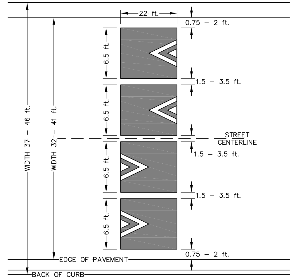
SPEED CUSHION DETAIL
